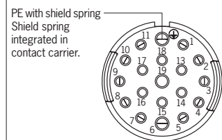
Fig. 3: Pin assignment for male plug View of connection side
