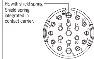
Fig. 2: Pin assignment for female plug View of connection side
